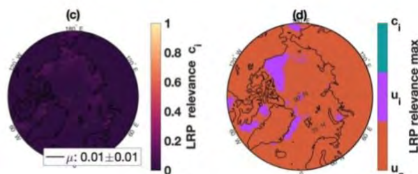
Figure 4: (a–c) Heat maps show the relevance of each of the inputs to an ML model for making predictions of sea-ice motion. These relevance heat maps are from an explainable machine learning (XML) method known as layerwise relevance propagation (LRP) applied to a CNN trained to make one-day predictions of sea-ice motion from inputs of wind velocity ( u_a ) in panel (a), ice velocity ( u_i ) in panel (b), and ice concentration ( c_i ) in panel (c). (d) Map showing which input is the most important predictor of sea-ice motion for the ML model at each location in the Arctic.
