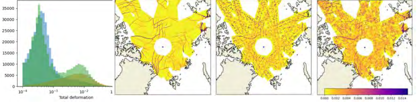
Figure 4. Maps of shear ( t ) computed from simulated velocities (1st column) and from Harmony denoised velocities using U^2 (2nd column) and U^3 (3rd column). PDFs of total deformation (blue – neXtSIM , orange – U^2 , green – U^3 ).
