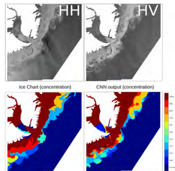
Figure 2: Example of a Sentinel-1 EW scene from the Scoresbysund Fjord in East Greenland. Upper left: Sentinel-1 HH polarisation. Upper right: Sentinel-1 HV polarisation. Bottom left: Manually drawn ice concentration chart (Greenland Ice Service). Bottom right: Ice concentration output from the CNN.
