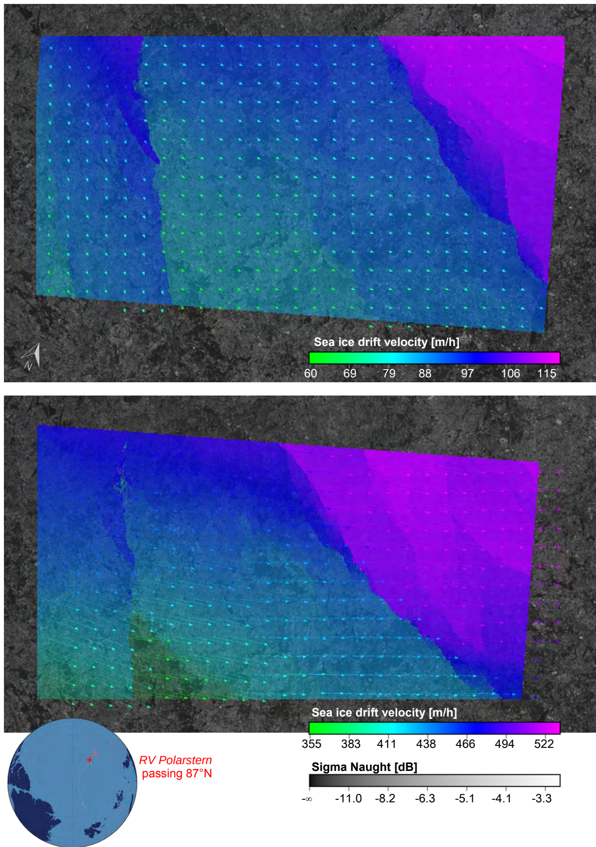
Figure 2: Examples for sea ice drift retrieval from TerraSAR-X data taken during MOSAiC expedition facing a storm event in late January 2020 in Arctic Ocean at 87°N. The background shows TerraSAR-X HH data from 2020/01/26 03:58 UTC (top) and 2020/01/27 03:41 UTC (bottom) in grey scale, calibrated to sigma naught. Overlaid colors represent retrieved sea ice drift velocity in 264 m resolution and arrows illustrate sea ice drift vectors (5 km spacing). The upper drift field is generated from TerraSAR-X acquisitions taken on 2020/01/25 and 2020/01/26, the lower from 2020/01/26 and 2020/01/27. Convergence and divergence zones become visible at the color jumps in the drift velocity map.
