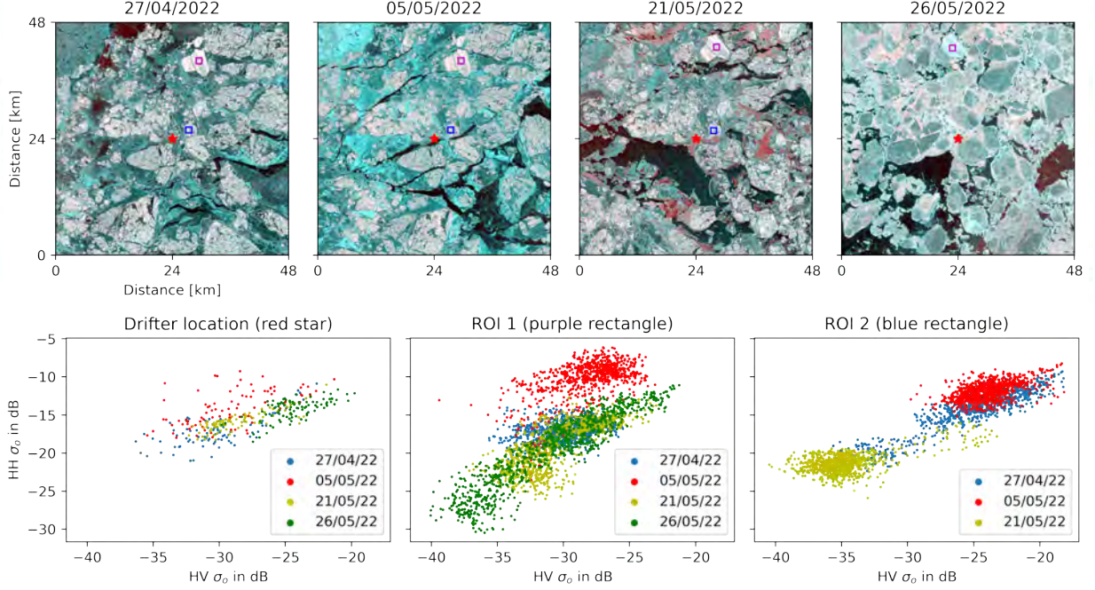
Fig. 2. Top: False-color RGB images (R-HV, G-HH, B-BH) of four S1 scenes that overlap with the drift trajectory of drifter 206754. The images are cropped to areas of 48x48 km around the drifter location at the time of image acquisition, as indicated in Figure 1 (right). The drifter location is indicated with a red star. Purple and blue rectangles indicate ROI's on distinct sea ice structures. Bottom: Scatterplots of HH versus HV backscatter values for a small area around the drifter location and for the two ROI's at the timestamps of the selected S1 images.
