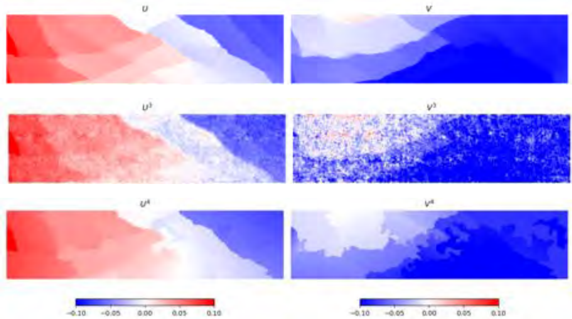
Figure 3. Velocity components after the steps of processing: U – initial range and azimuth components, U^3 – low-pass and anisotropic diffusion, U^4 – clustering.
