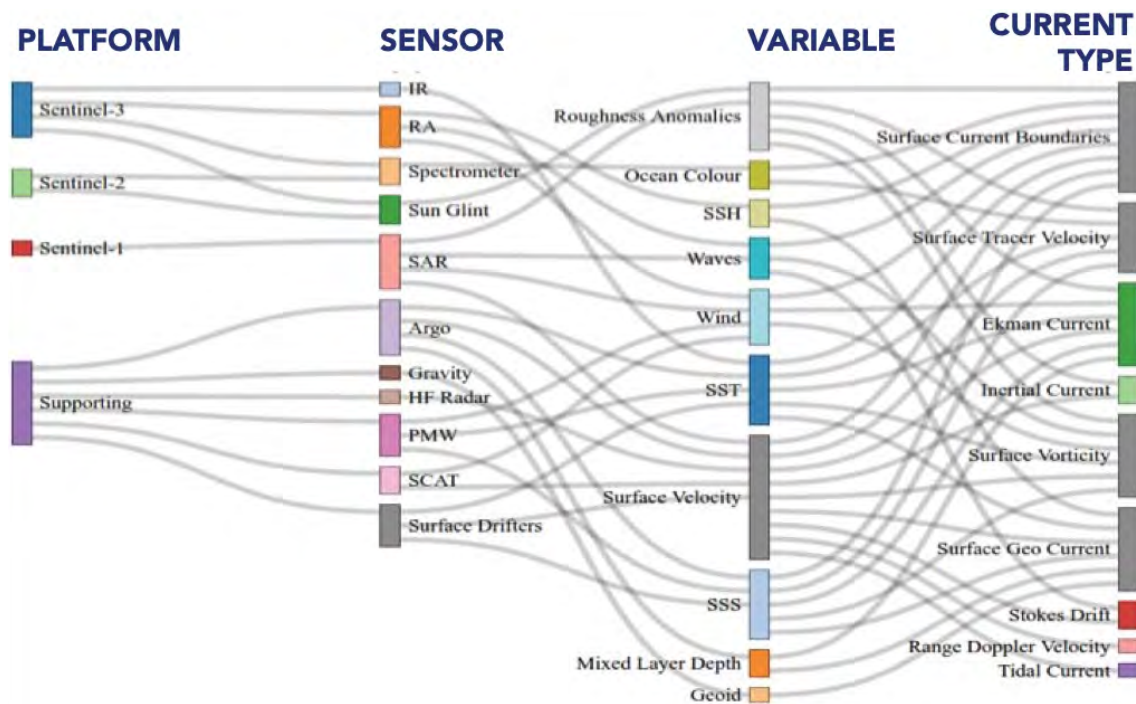
Figure 1. Example of satellite sensor synergy for upper ocean current monitoring based on the Sentinel-1,-2,-3 combinations of infrared (IR) and microwave radiometer (PMW); imaging spectrometer; radar altimeter (RA); SAR-based surface roughness and range Doppler velocity; scatterometer based surface roughness and wind field; and Visible-derived sun-glint.
