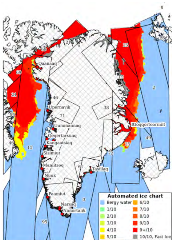
Figure 3: Example of a concentration mosaic of several days of Sentinel-1 imagery processed by the CNN. The mosaic was generated on November 7th 2022.
