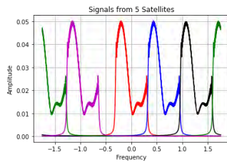
Figure 1 – Frequency Response for five satellites with the separation of 4 km between them
