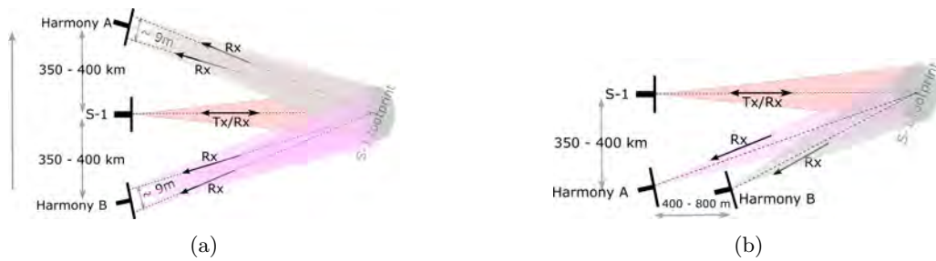
Figure 1: Satellite configurations of the Harmony mission. (a) Stereo configuration, (b) Across-track interferometric configuration.
