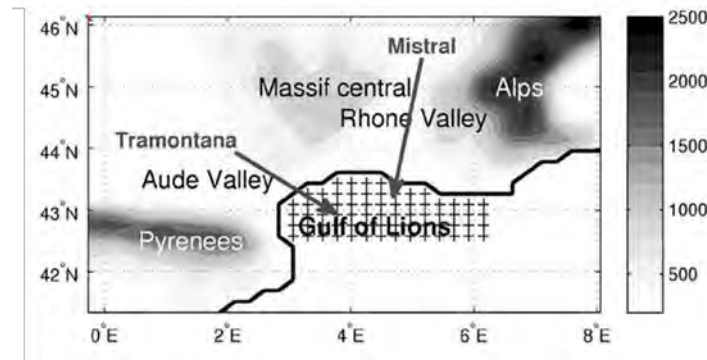
Fig. 1. Topography of the Gulf of Lion (adapted from (Omrani et al., 2017))
