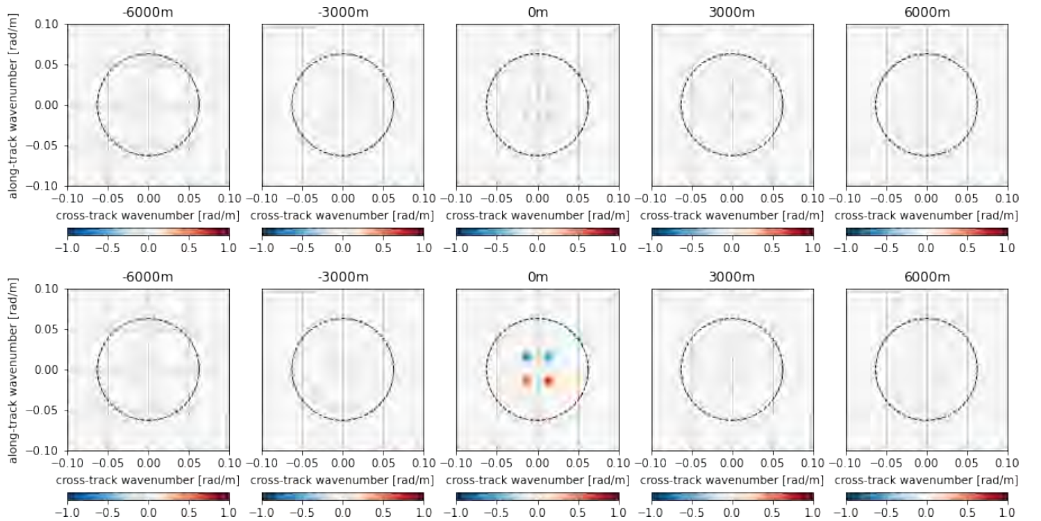
Figure 2: Imaginary values of numerically modeled satellite nadir altimetry cross-spectra based on ten realizations at five along-track distances. The input consists of a swell system with a peak wavelength of 277 m propagating at 45 (top) and 225 (bottom) degrees from cross track (right), and a wind-sea system based on a wind speed of 10 m/s, a fetch of 200 km at a mean direction of 45 degrees from cross track.
