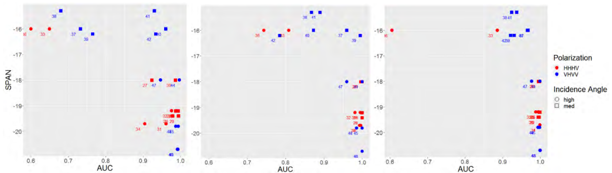
Figure 4: Detector comparison results for dual cross-pol data.
