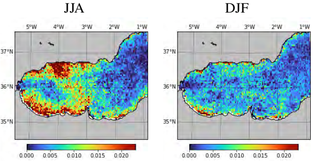
Fig. 3. Biological slick detection probability (restricted to points with wind speed between 6.5 and 12 m/s) during summer (left) and winter (right) in the Alboran Sea between 2015 and 2022.
