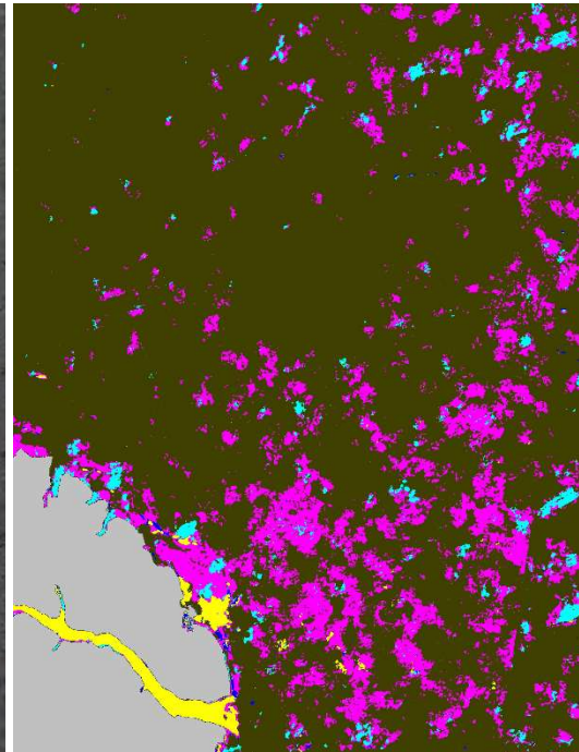
Fig. 3: Sea ice classification based on the two SI acquisitions used for the sea ice classifications in Fig. 1. The unlikely presence of “young ice” over Lincoln Sea on 6 th Dec. gets corrected in most parts. Colour legend see Fig. 1 top right.
