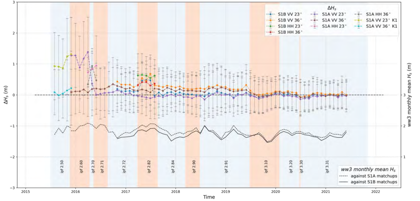
Figure 1: (left y-axis) \Delta H_s (Sentinel-1 – WW3) monthly mean and standard deviation time series of Sentinel-1A/B wave mode data as a function of platform, polarisation, and incidence angle, and (right y-axis) WW3 monthly mean H_s computed against Sentinel-1 A A and B matchups. Sentinel-1 IPF version evolution through time is highlighted.
