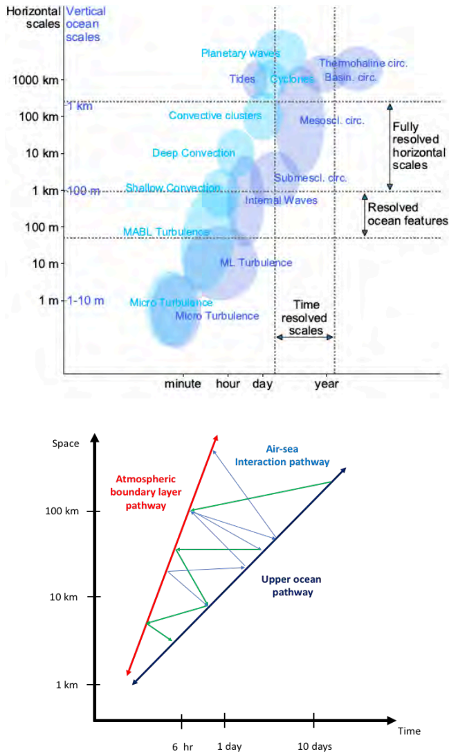
Figure 5. (upper) Schematic illustration of the time-space scales of dominant ocean-atmosphere phenomena and interactive processes, including a range of vertical scales where these processes occur. (lower) Indications of the multiple pathways of atmosphere-ocean interactions.
