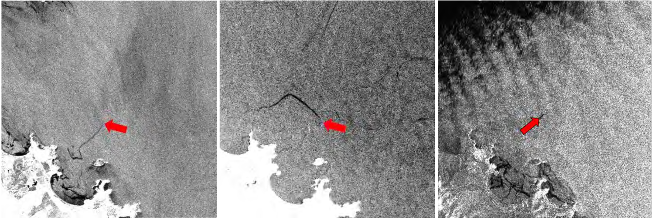
Figure 2. Three examples of SAR images of the Mopang site, acquired in 2018, 2016, and 2006 (left to right) and showing manifestations of the heavy fuel spill; image dimensions 16.6 km \times 16.9 km. Left: ALOS-2 PALSAR-2 image acquired on 8 July 2018; middle: Sentinel-1A SAR-C image acquired on 9 September 2016; right: ENVISAT ASAR image acquired on 15 September 2006. Red arrows mark the position of the SS Mopang .
