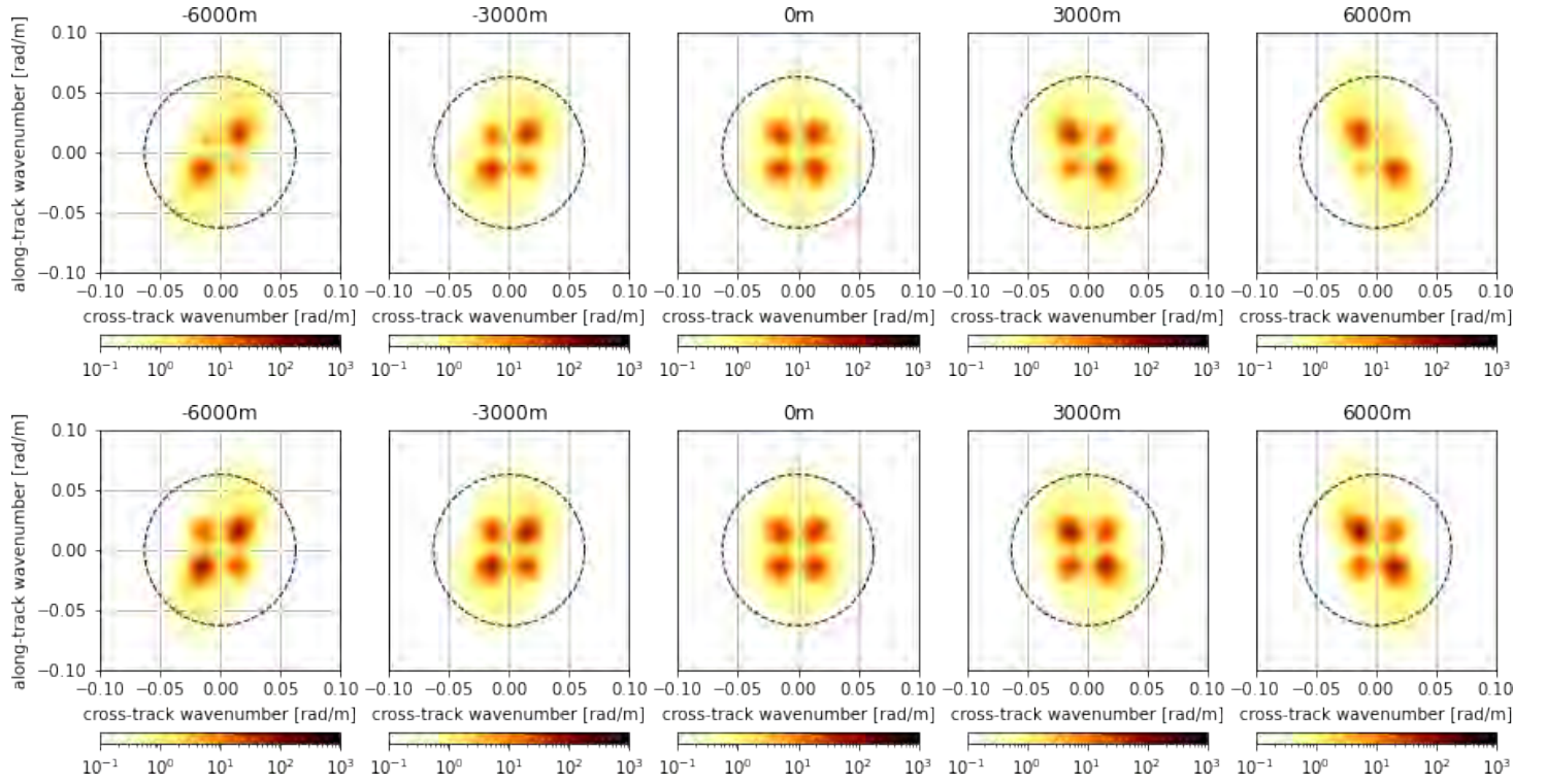
Figure 1: Absolute values of numerically modeled satellite nadir altimetry cross-spectra based on ten realizations at five along-track distances. The inputs consist of swell systems with a peak wavelength of 277 m propagating at 45 (top) and 135 (bottom) degrees from cross track (right), and a wind-sea system based on a wind speed of 10 m/s, a fetch of 200 km at a mean direction of 45 degrees from cross track.
