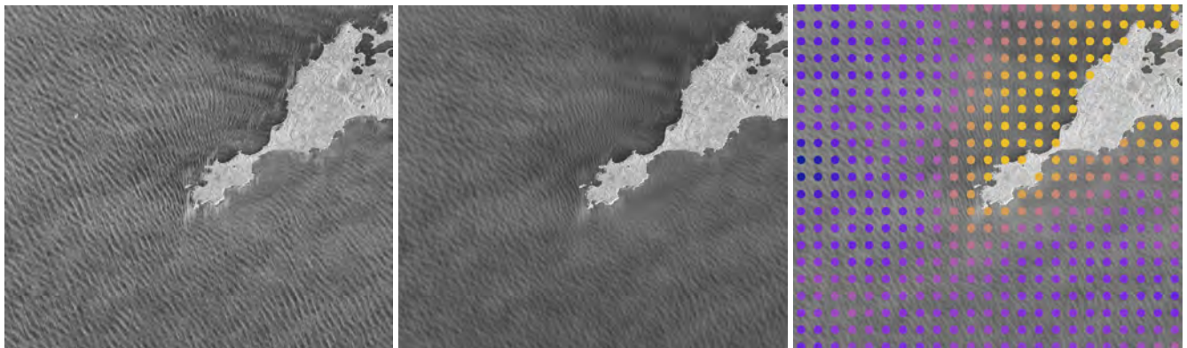
Fig. 2: Example of a wave pattern and water depth extraction result for an area at Rottneest Island (Australia), after [16]. Left: TerraSAR-X Sliding Spotlight Mode image from 20 Oct 2009, 11.7 \text{ km} \times 10.4 \text{ km} , integration time = 1.22 s; center: extracted wave signatures; right: extracted depths between 60 m (blue) and 0 (yellow), grid spacing = 512 \text{ m} \times 512 \text{ m} .
