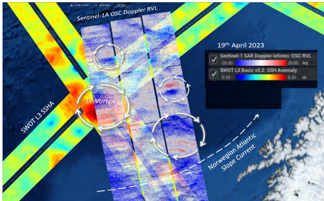
Figure 3. Collocated SWOT sea surface height and Sentinel-1 range Doppler velocity in the Lofoten Basin acquired on 19 April 2023. White circles mark presence of cyclonic and anticyclonic eddies. Colour scale marks Sentinel-1 Doppler shift (Hz) and SWOT SSH (m)
