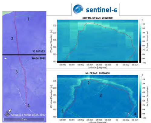
Figure 3. Sentinel-6 radargrams for pass #95 from Unfocussed and Fully focussed processing highlighting the features leads that can be seen.
