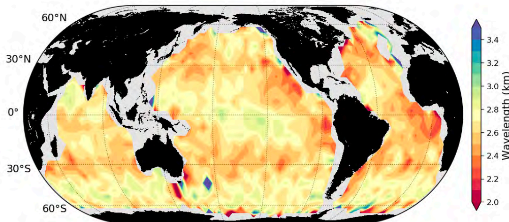
Figure 4. Global distribution of extracted roll wavelengths from the most energetic peak of the identified WV SAR images. Colour donates the average in 5° by 5° grid boxes. (Courtesy of C. Wang.)
