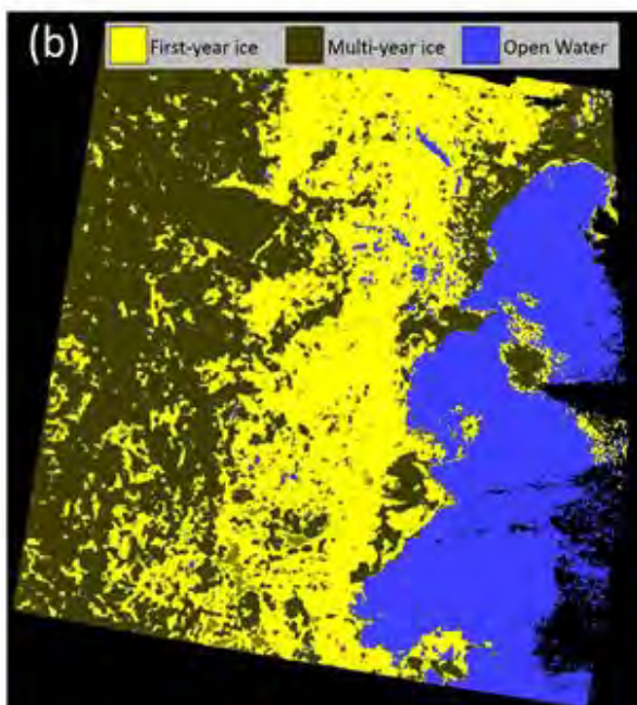
Figure 5. Example classification results. (a) SAR classification using only S1 data, (b) fused classification using SAR data and an SLSTR classification. Most open water areas are identified correctly by the fused classification. Note that the same cloud mask is applied to both scenes, causing the frayed black areas on the right.
