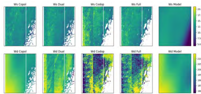
Fig. 2 Results for S1A IW GRDH ISDV 20220528T055454. Upper row is wind speed and lower is wind direction, using the four different inversions and the ECMWF model data.
