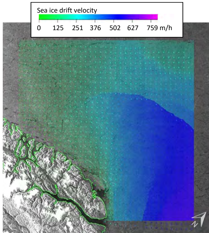
Fig. 2: Sea ice drift estimated from the two SI acquisitions used for the sea ice classifications in Fig. 1. Grey scales show SI HH data from 7 th Dec. 2021. Overlaid colours represent retrieved sea ice drift velocity in 500 m resolution and arrows illustrate sea ice drift vectors (10 km spacing).
