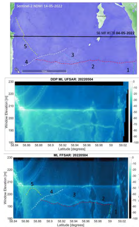
Figure 2. Sentinel 6-radargrams for pass #178 from Unfocussed and Fully focussed processing highlighting the leads that can be seen
